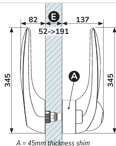
Overlapping door
