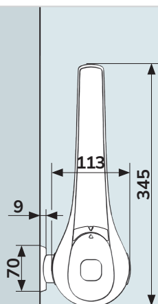
Internal fastener
